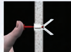
Insert key to pop anchor open behind hollow wall (not necessary for thick or solid walls) Do not force or hammer key.
