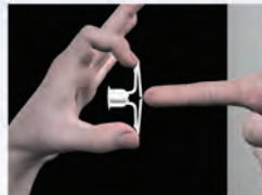
Drill 5/16" (8mm) hole. Fold anchor in middle.
